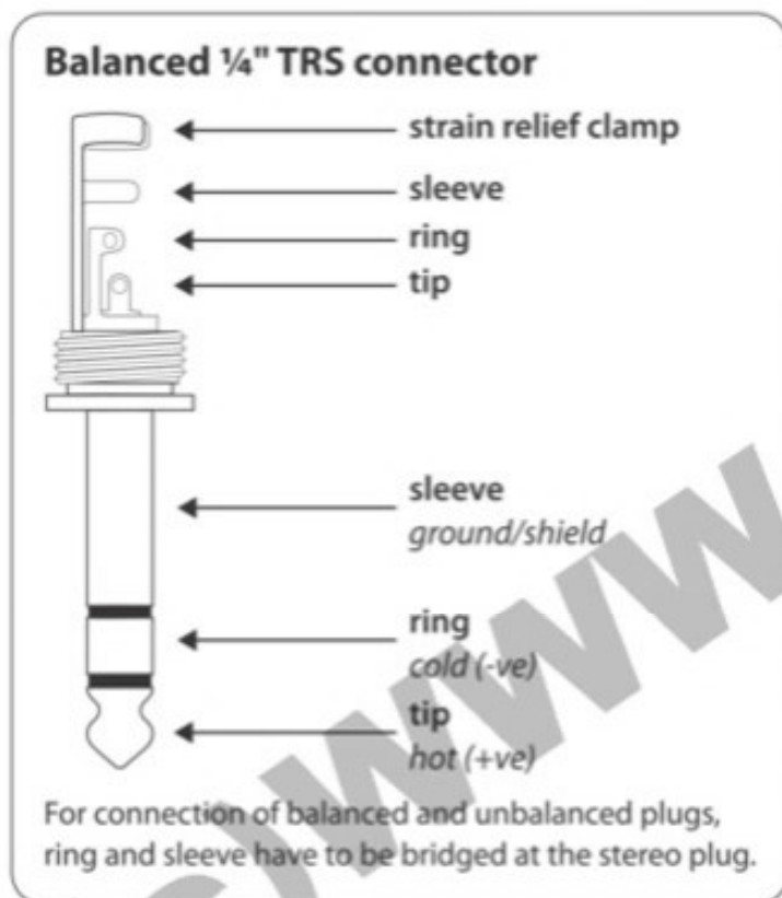
Fig. 4.2: TRS stereo connector
